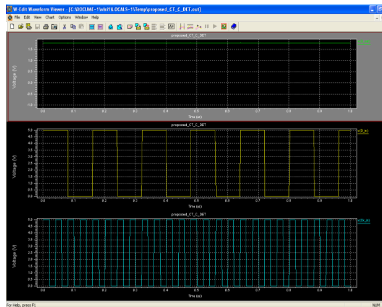
Figure 7: The output of the proposed CT_CDET
