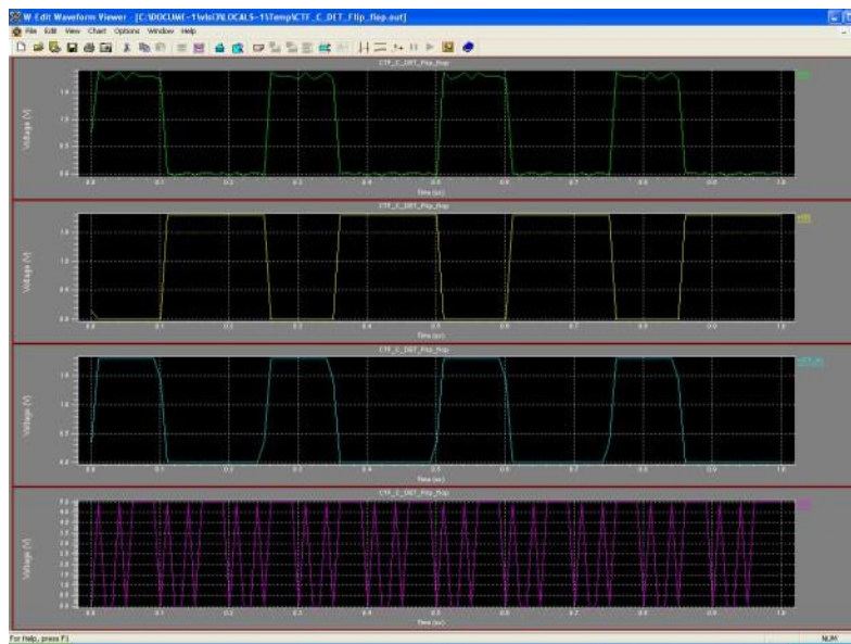
Figure 6: output of the Existing conditional-toggle CTF_C DET flip-flop
