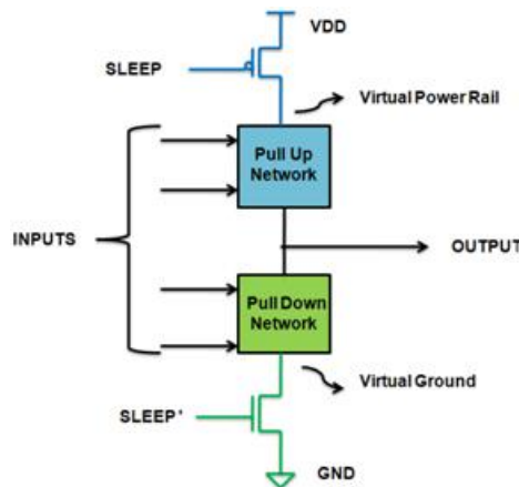
Figure 3: Schematic representation of Power gating technique
