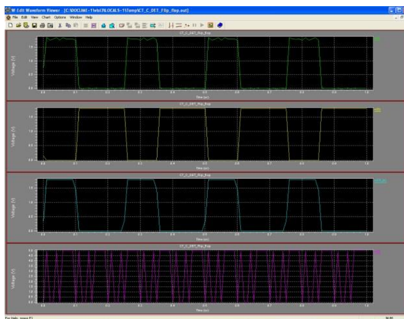
Figure 5: output of the Existing conditional-toggle
