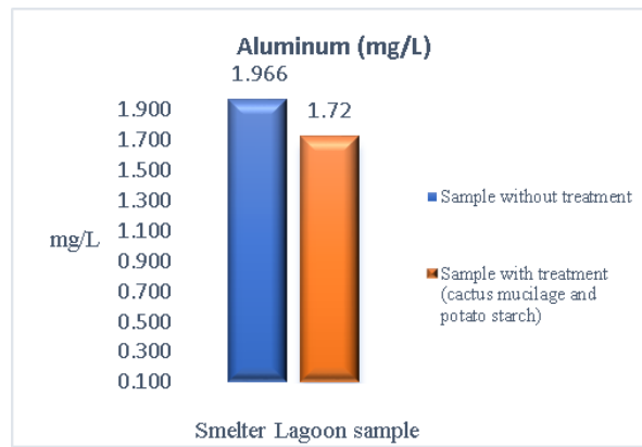
Fig. 4. Aluminium removal.
