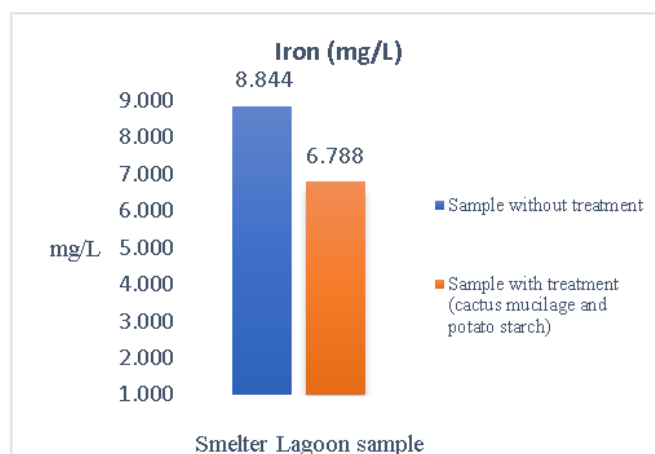
Fig. 6. Iron removal.
