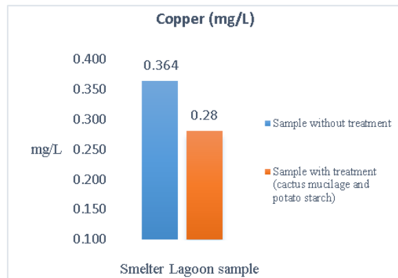
Fig. 5. Copper removal.
