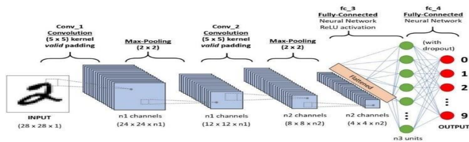
Figure 2. Layers of CNN
