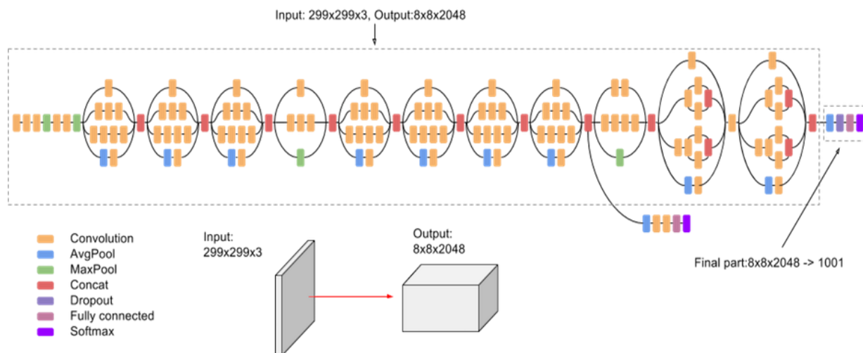
Figure 3 A high-level diagram of CNN model
